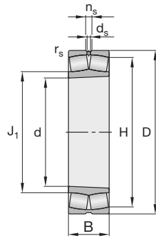
tapered bore
