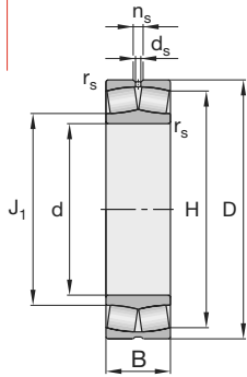
cylindrical bore
